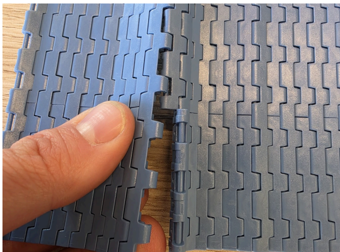
Joining and unzipping belt sections. Clip together, no joiners required.
